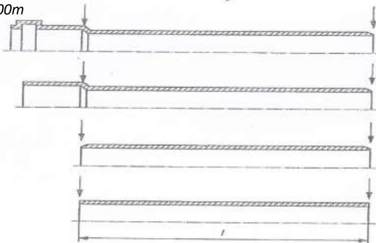
Figure 1 — Points of measurement for nominal pipe lengths
